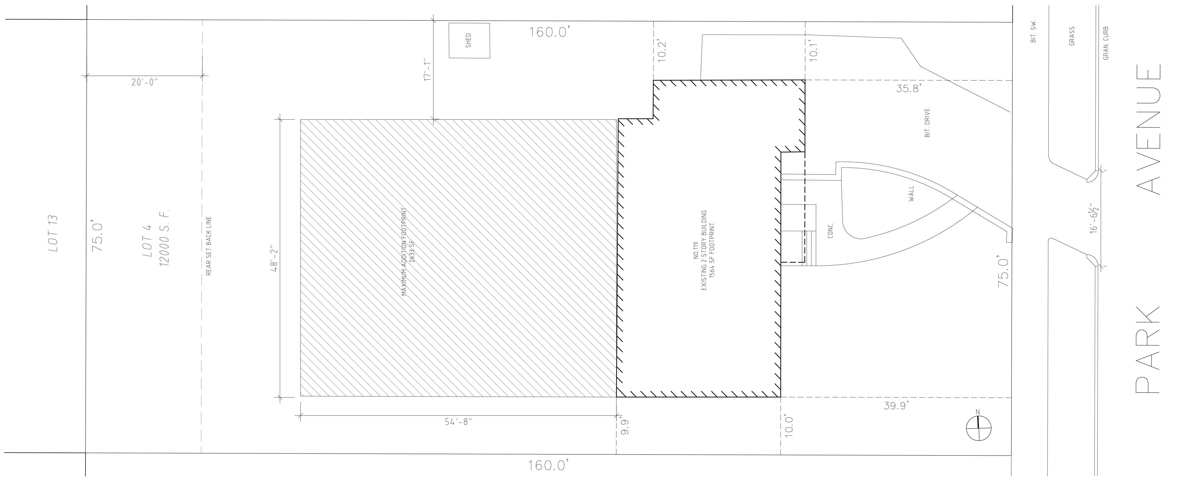
2 MAXIMUM ADDITION FOOTPRINT 1/8" = 1'
